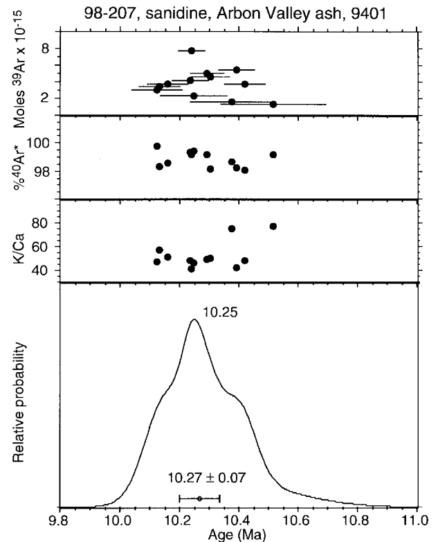
Figure 6. Age-probability distribution diagram (Deino and Potts, 1990) of single-crystal laser-fusion analyses of sanidine crystals from ash low in the Cache Valley member of the Salt Lake Formation (lower panel). The age and K/Ca ratio shows that this tuff is correlative with tuff of Arbon Valley. Upper panels are auxiliary plots showing moles of K-derived ^{39}\text{Ar} , percent radiogenic yield, and K/Ca ratios. Upper panel also shows 1 sigma analytical uncertainty for each crystal. Lower panel shows weighted mean age and 2 sigma uncertainty.
