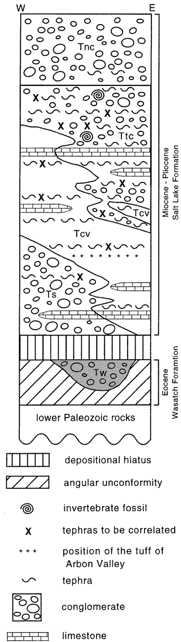
Figure 8. Schematic stratigraphic column of the Tertiary units within the Deep Creek half-graben. Abbreviations for members of the Tertiary Salt Lake Formation are: Tcv = Cache Valley, Tnc = New Canyon, Ts = Skyline, Ttc = Third Creek, Tw = Tertiary Wasatch Formation.
