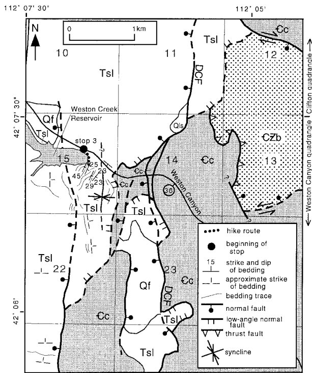
Figure 10. Photogeologic map showing the area around Stop 3. Section lines and numbers are shown for reference. The geology of the pre-Tertiary rocks is modified from Murdock (1961). Cc = Cambrian carbonate rocks, CZb = Neoproterozoic Brigham Group, DCF = Deep Creek fault, Qf = Quaternary alluvial fan deposits, Qls = Quaternary landslide deposit, Tsl = Tertiary Salt Lake Formation.
